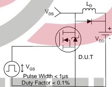
Fig 14a. Switching Time Test Circuit
